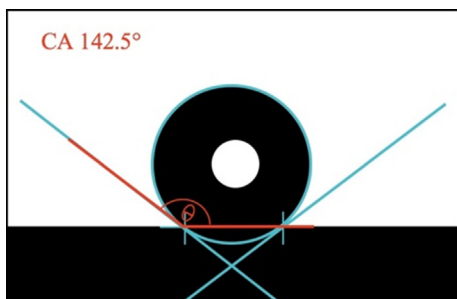
Fig. 4 Water contact angle for grafted silica sand hollow fibre ceramic membrane.
