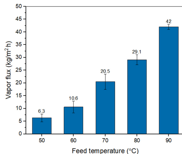
Fig. 8 Feed temperature effect on the water vapor flux of surface modified SSCHFMs (NaCl concentration = 8 g/L, permeate temperature = 10 °C, feed flow rate = 30 L/h) (number of samples, n = 3 ).
