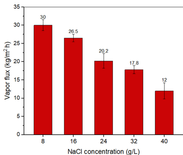
Fig. 7 Water vapour flux of grafted SSCHFMs at different NaCl concentrations (10 °C permeate temperature, 80 °C feed temperature, 30 L/h feed flow rate) (number of samples, n = 3 ).
