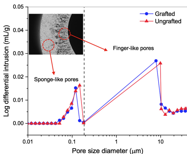
Fig. 6 Pore size distribution for SSCHFMs before and after surface modification.
