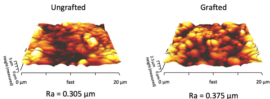
Fig. 5 Three-dimensional AFM images of ungrafted and grafted SSCHFMs.
